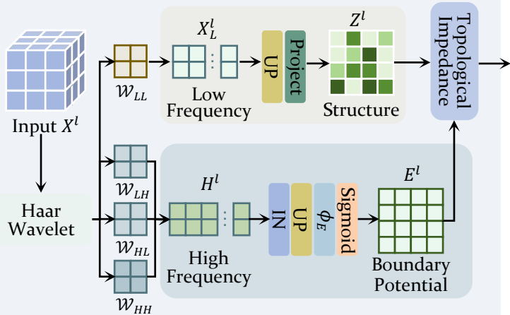
Frequency-Topology Conductance Field (FTCF)
