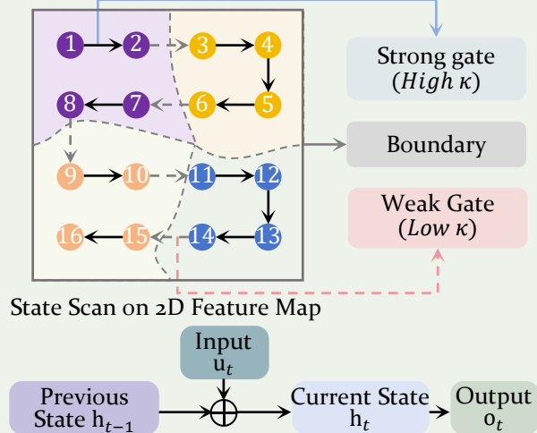
Conductance-Gated State Scan (CGSS)
