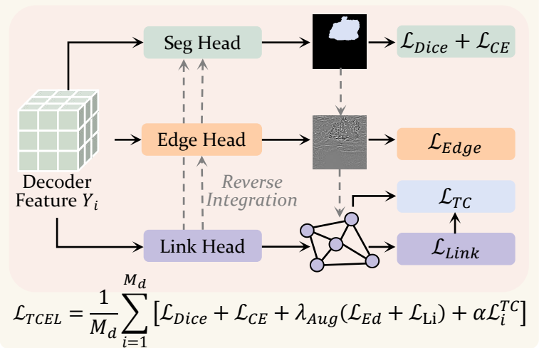
Topology-Consistent Ensemble Learning (TCEL)
