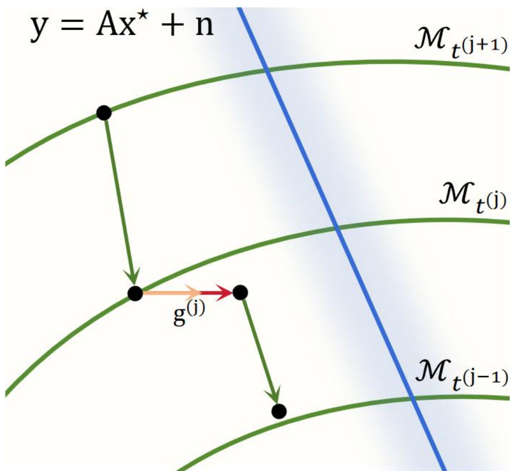
(a) Standard Sampling (Gradient-Only Correction)
