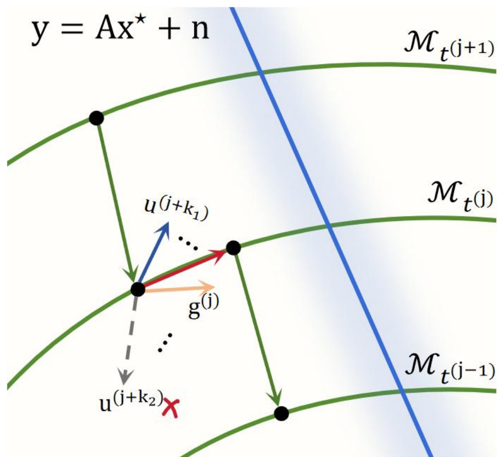
(b) TrajSPC Sampling (Trajectory Subspace Proximal Correction)
